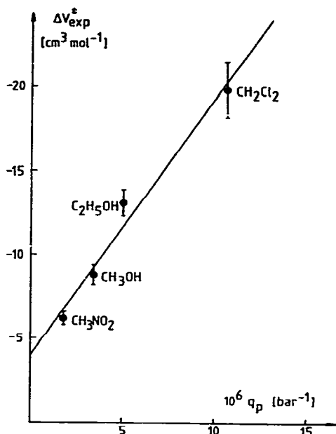
Fig. 7. The relationship between the volume of activation and the q_p parameter for the reaction of \text{trans-Pt(py)}_2(\text{Cl})\text{NO}_2 with pyridine [54].
