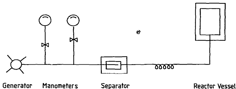
Fig. 1. Diagram of high pressure apparatus.
