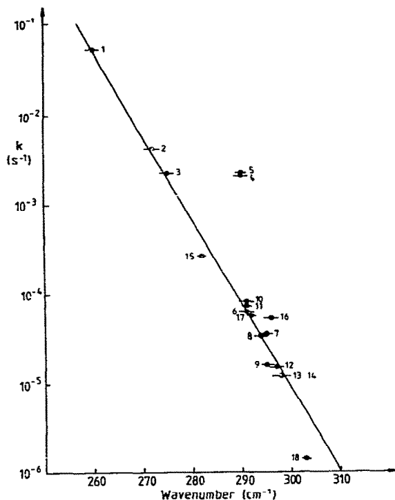
Fig. 3. Correlation between \log k of the hydrolysis reactions of \text{Co}(\text{N}_4)\text{Cl}_2^+ and the N—Co—N deformation frequency [101,104]. Key: 1, trans -[Co(tmd) 2 Cl 2 ] \text{ClO}_4^{\text{a}} ; 2, trans -[Co(sbn) 2 Cl 2 ] \text{ClO}_4^{\text{a}} ; 3, trans -[Co(ibt) 2 Cl 2 ] \text{ClO}_4^{\text{a}} ; 4, trans -[Co(NH 3 ) 4 Cl 2 ] \text{Cl}^{\text{a}} ; 5, trans -[Co(NH 3 ) 4 Cl 2 ] \text{Cl}^{\text{b}} ; 6, trans -[Co(pn) 2 Cl 2 ] \text{ClO}_4^{\text{a}} ; 7, trans -[Co(en) 2 Cl 2 ] \text{ClO}_4^{\text{a}} ; 8, trans -[Co(en) 2 Cl 2 ] \text{Cl}^{\text{b}} ; 9, trans -[Co(Meen) 2 Cl 2 ] \text{Cl}^{\text{b}} ; 10, trans -[Co(Eten) 2 Cl 2 ] \text{Cl}^{\text{b}} ; 11, trans -[Co(Pren) 2 Cl 2 ] \text{Cl}^{\text{b}} ; 12, trans -[Co(2.3.2-tet)Cl 2 ] \text{Cl}^{\text{a}} ; 13, trans -[Co(RS-2.3.2-tet)Cl 2 ] \text{Cl}^{\text{b}} ; 14, trans -[Co(RS-2.3.2-tet)Cl 2 ] \text{ClO}_4^{\text{b}} ; 15, trans -[Co(RR,SS-2.3.2-tet)Cl 2 ] \text{ClO}_4^{\text{c}} ; 16, trans -[Co(2.3.2-tet)Cl 2 ] \text{ClO}_4^{\text{a}} ; 17, trans -[Co(3.2.3-tet)Cl 2 ] \text{Cl}^{\text{b}} ; 18, trans -[Co(cyclam)Cl 2 ] \text{Cl}^{\text{a}} . a 0.1 M HNO 3 ; b 0.01 M HNO 3 , \mu = 0.1 M; c pH = 2, \mu = 0.014 M.
